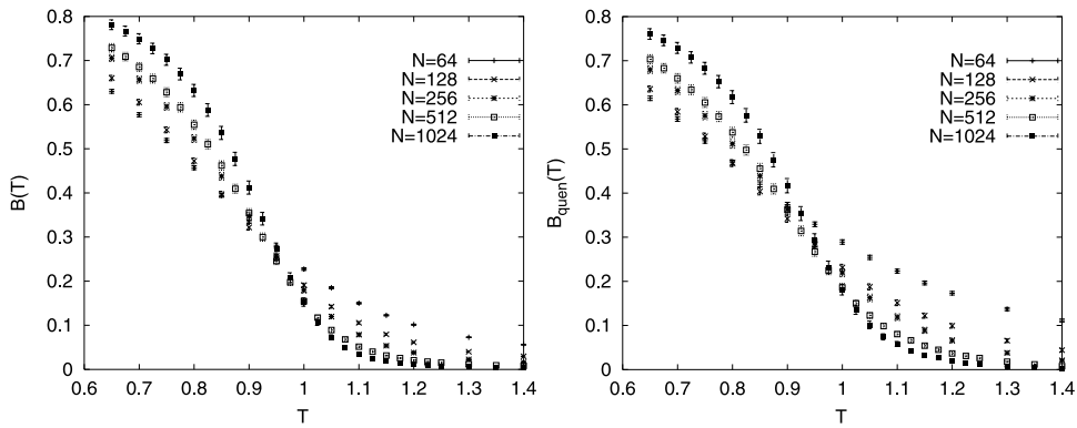
Figure 4. The Binder parameter from the equilibrium P(q) (left) and from the quenched one (right) as a function of temperature for different system sizes.
