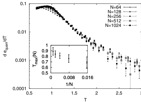
Figure 10. The quenched energy (left) and its derivative with respect to the temperature (right) as a function of T for the different system sizes N . In the inset on the right, the temperature corresponding to the maximum of de_{quench}/dT is plotted as a function of 1/N .
