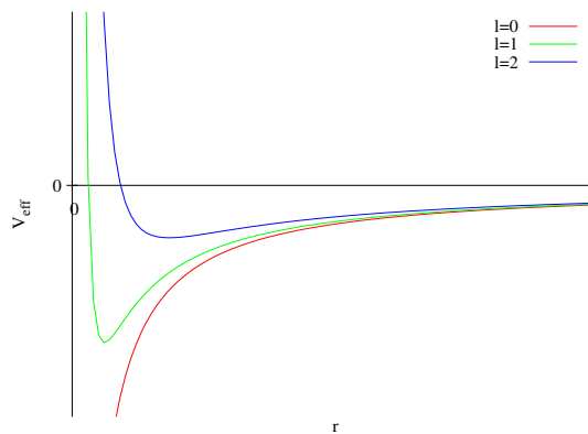
ABBILDUNG 3.1: V_{eff}(r) = -\frac{q^2}{r} + \frac{l(l+1)}{2mr^2}
